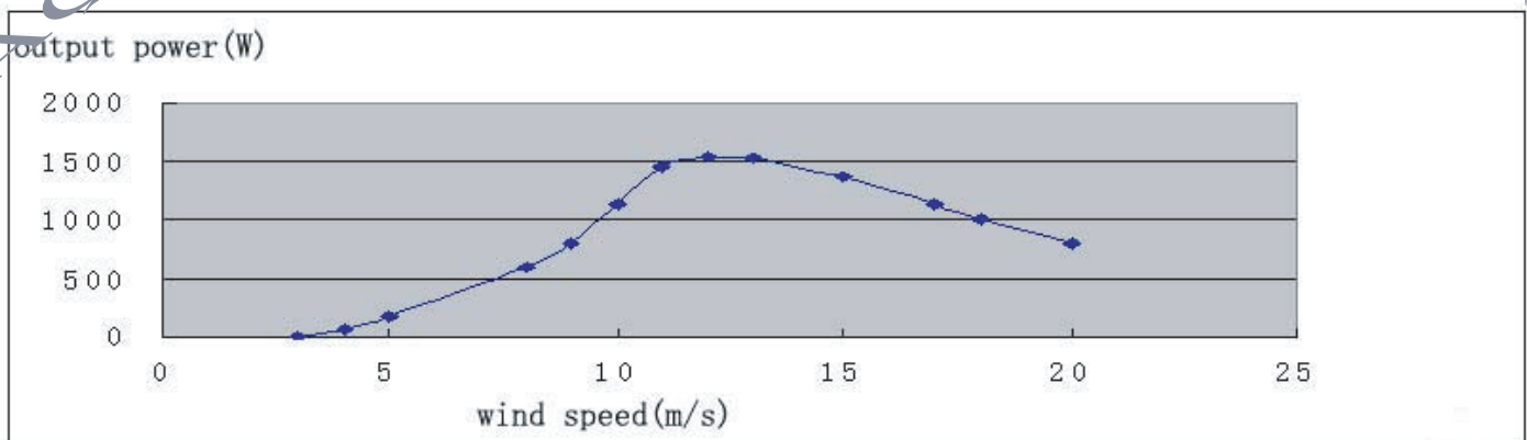
1kW wind generator power curve
