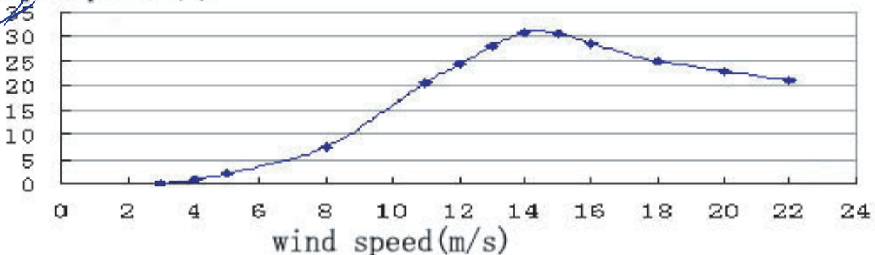
20kw wind generator power curve
