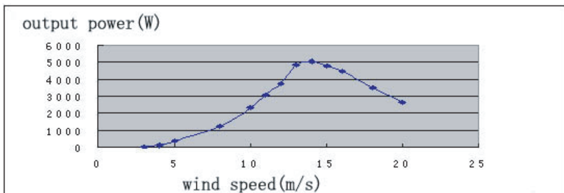
3KW wind generator power curve
